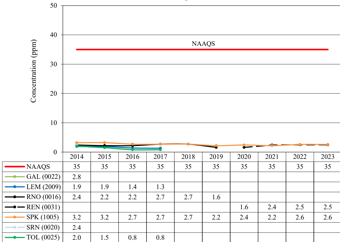
Figure 18 CO (1-hour) Design Values
