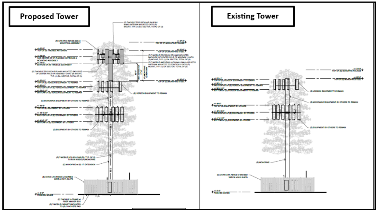
Tower Plans- Proposed & Existing
