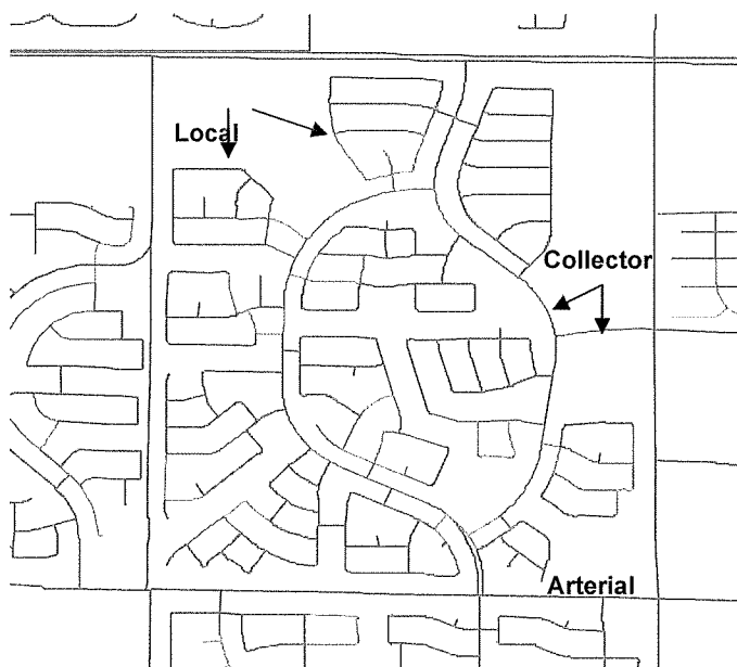
Figure 14: Road Hierarchy Example
